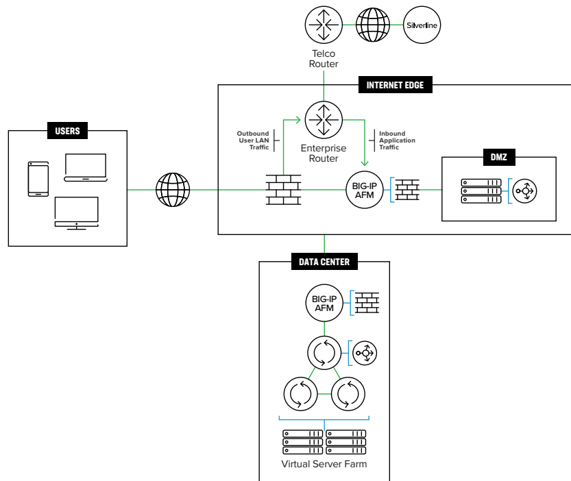
Figure 1: AFM DDoS Protection supports off-loading of larger volumetric attacks to up stream routers or routing traffic to Silverline for removal of DDoS traffic.
