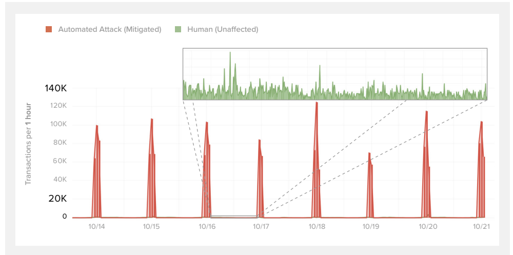
Figure 5: Forgot User ID attack against a Global 2000 F5 customer
